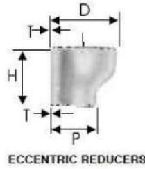
ECCENTRIC REDUCERS
